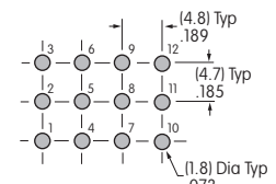
Four Pole
